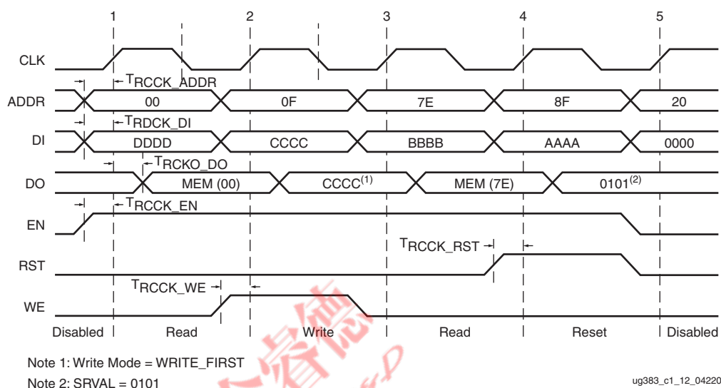
Figure 13: Block RAM Timing Diagram
